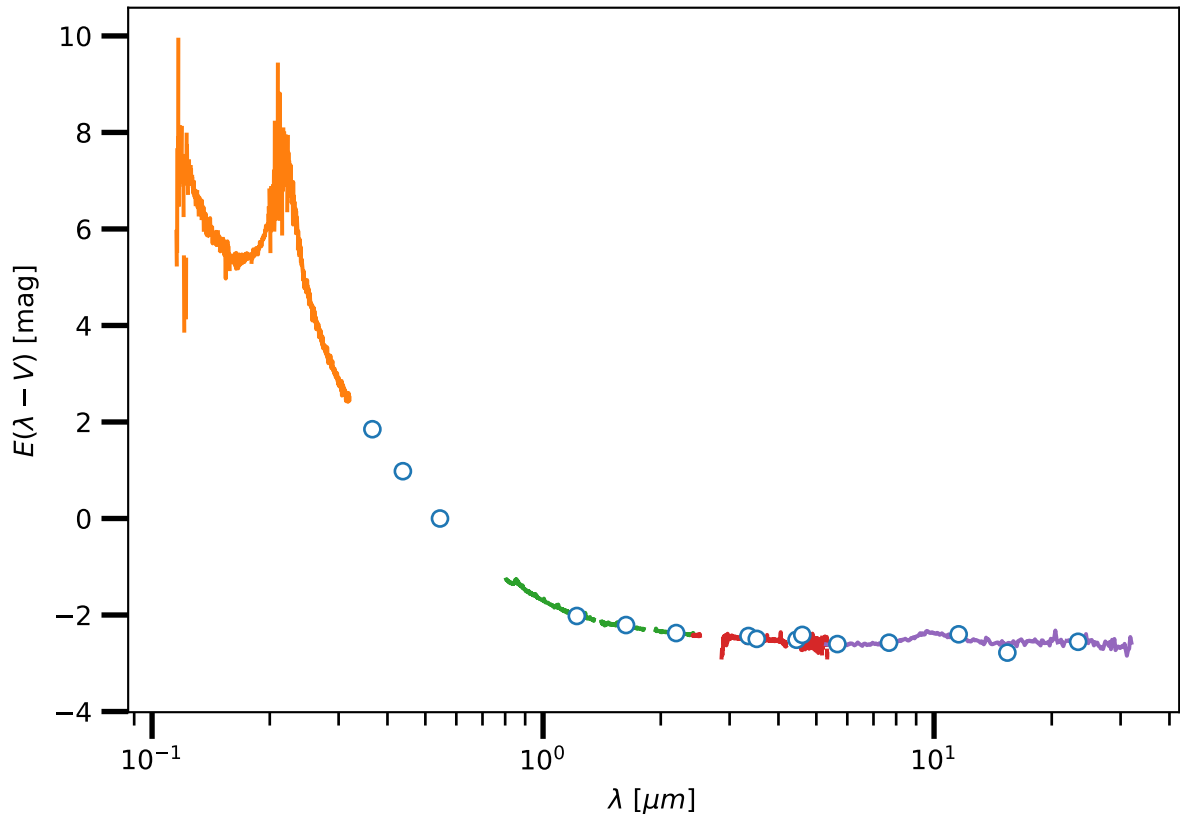
HD229238/HD204172 extinction
